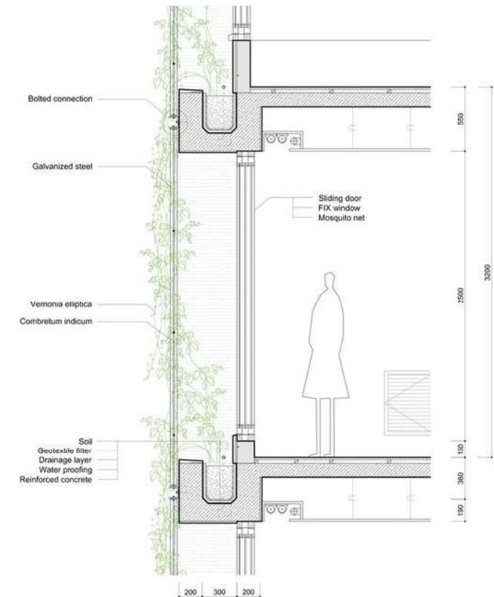
Section Detail
