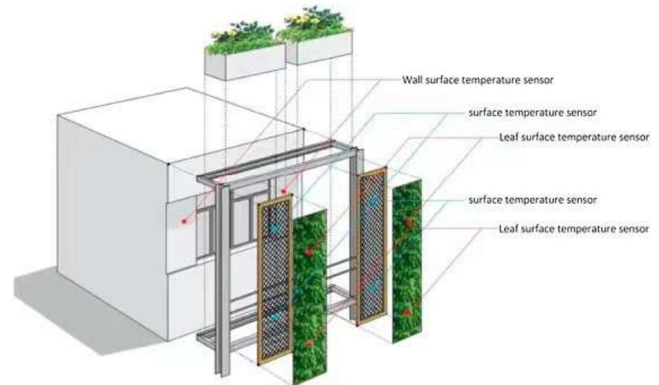
Steel structure stainless steel (2mm~4mm)
